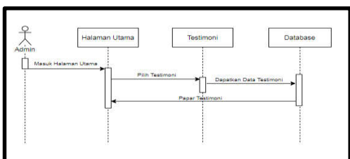
Gambar 4.10. Sequence Input Data Testimoni
