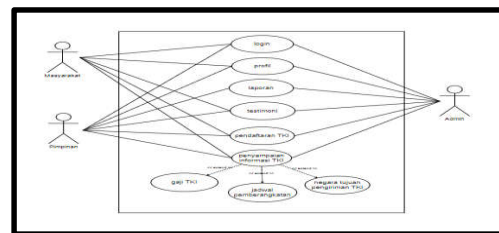
Gambar 4.1. Use Case Diagram
