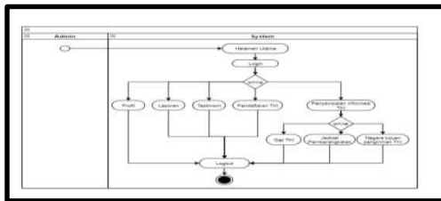
Gambar 4.2. Activity Diagram Admin
